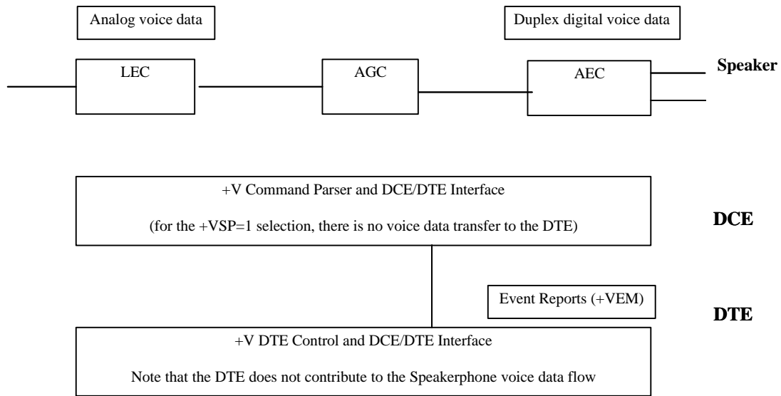
Figure 3 – PSTN ↔ DCE Microphone and Speaker (+VSP=1)
