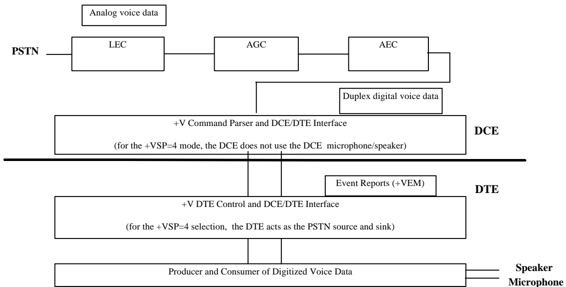
Figure 6 -- DCE ↔ DTE Microphone and Speaker (+VSP=4)
